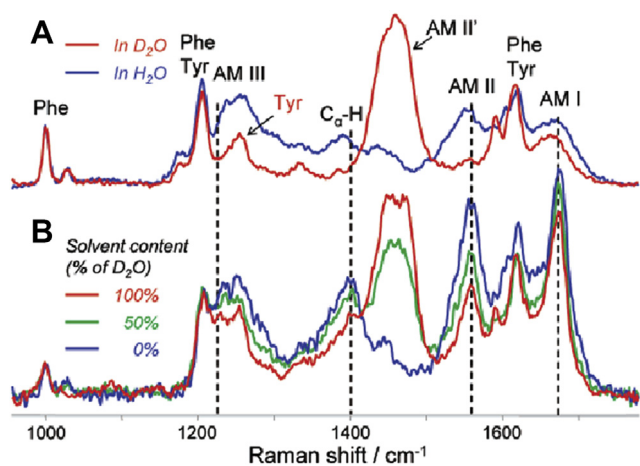
Fig. 3. Deep UVRR spectra of (A) thermally denatured hen egg white lysozyme in H_2O (blue) and D_2O (red), and (B) lysozyme fibrils in H_2O (blue), 50% D_2O/H_2O mixture (green), and 100% D_2O (red). Spectra were collected using an excitation wavelength of 197 nm. Adapted with permission from Ref. [42]. Copyright 1982 American Chemical Society.
