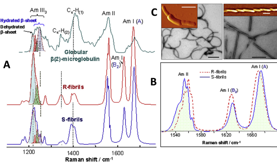
Fig. 4. (A) Deep UVRR spectra of antiparallel \beta -sheet-rich globular \beta_2m (green) and cross- \beta -core of R-fibrils (red) and S-fibrils (blue). The cross- \beta -core spectra were extracted from the data sets obtained for partially deuterated fibrils using a Bayesian approach. (B) Amide I and amide II region of R- and S-fibril Raman spectra. (C) EM (black-and-white) and AFM (orange-yellow) images of S-fibrils (left) and R-fibrils (right). Scale bars correspond to 0.2 \mu m . Adapted with permission from Ref. [46]. Copyright 2016 American Chemical Society.
