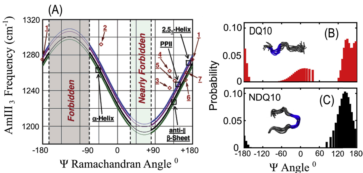
Fig. 1. (A) Sinusoidal dependence of the AmIII 3 S band frequency on the \Psi Ramachandran angle. The four curves show the correlation for peptide backbone in different environments: (blue) fully solvated, (purple) only C=O groups involved in peptide-peptide hydrogen bonding, (black) only N-H groups involved in peptide-peptide hydrogen bonding, and (green) N-H and C=O groups both involved in peptide-peptide hydrogen bonding. The red diamonds show experimental data points for small crystalline peptides: 1. Ala-Asp, 2. Gly-Ala-Leu, 3. Val-Glu, 4. Ala-Ser, 5. Val-Lys, 6. Ser-Ala, and 7. Ala-Ala. Figures B and C show \Psi angle distributions of the small monomeric polyQ peptides DQ10 (B) and NDQ10 (C) as derived from the AmIII 3 S - \Psi angle correlation. The insets show the structural models of the monomeric peptides produced from UVRR measurements and metadynamics simulations. Panel (A) was adapted with permission from reference 14. Copyright 2006 American Chemical Society. Panels B and C were adapted with permission from reference 32. Copyright 2017 American Chemical Society.
