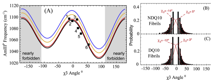
Fig. 2. (A) Dependence of the \text{AmIII}_3^{\text{P}} frequency on the Gln \chi_3 torsion angle. The black squares show experimental data for crystalline Gln-like compounds 1 L-Gln, 2 Gly-Gln, 3 D-Gln, 4 Gln t -butyl ester, 5 N-Acetyl-Gln, and 6 Ser-Asn. (B) and (C) show Gln side chain \chi_3 angle distributions for polyQ fibrils made from monomeric NDQ10 (B) and DQ10 (C) as derived from the \text{AmIII}_3^{\text{P}} - \chi_3 angle dependence. Panel (A) was adapted with permission from reference 9. Copyright 2015 American Chemical Society. Panels B and C were adapted with permission from reference 22. Copyright 2017 American Chemical Society.
