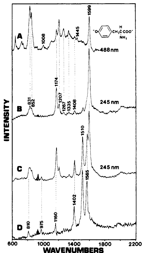
Figure 3. Raman spectra of tyrosinate ion (pH 12): (A) normal Raman spectra of tyrosinate with a CW laser (a water background spectrum has been subtracted, power = 900 mW, spectral bandpass = 2.5\text{ cm}^{-1} , the tyrosinate concentration is 100 mM); (B) UVRR spectrum of a 5 mM tyrosinate solution at 245-nm excitation using a 20-Hz Nd-Yag laser at 3-mW average power (the laser beam was focused above the sample); (C) same conditions as B but with the laser beam focused in the sample; (D) spectrum of the tyrosinate photoinduced transient obtained as the difference spectrum between B and C. Perchlorate ion is indicated by shading. Spectral bandpass = 12\text{ cm}^{-1} .
