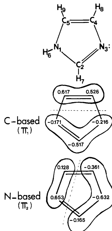
Figure 9. Molecular orbital coefficients of the π 1 and π 2 molecular orbitals of imidazole as determined by Del Bene and Jaffe. 32 Dotted lines depict nodal planes.
