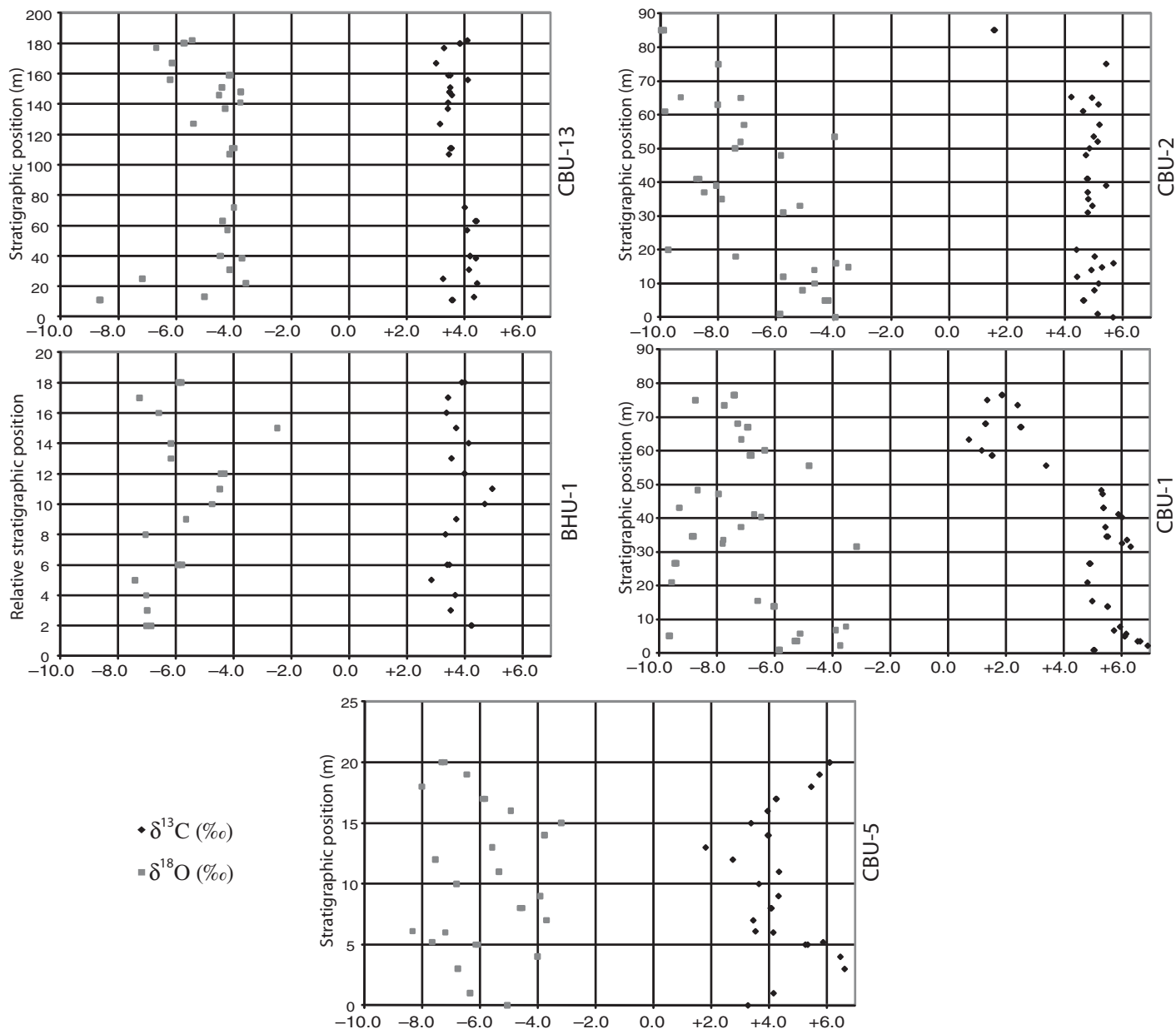
Figure 6. The \delta^{13}\text{C} and \delta^{18}\text{O} data versus stratigraphic position (note different vertical scales for each section) for five Baxa Group dolomite sections. Section BHU-1 is stratigraphically below section CBU-13 along the Trashigang-Samdrup Jongkhar road, section CBU-1 is stratigraphically below section CBU-2 in the Kuru Chu valley, and section CBU-5 is located in a different thrust sheet, farther south in the Kuru Chu valley (Fig. 2). Note consistent high positive \delta^{13}\text{C} values, generally between +3‰ and +6‰. Data for individual analyses are shown in Table DR3 [footnote 1].
