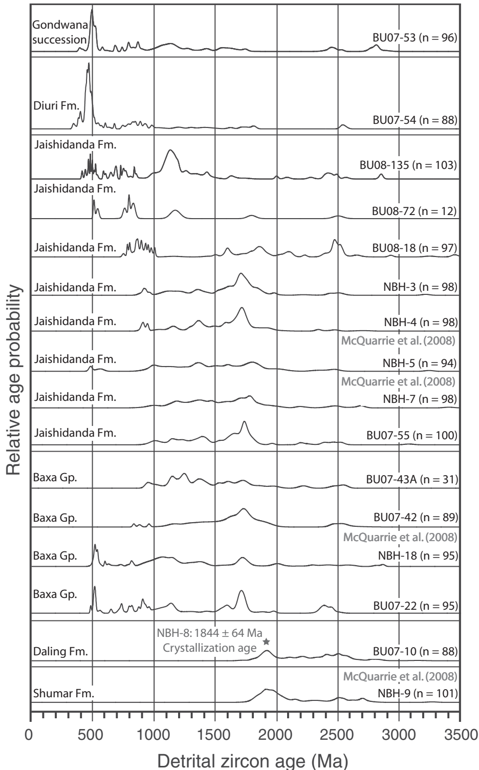
Figure 5. U-Pb detrital zircon age spectra of Bhutan Lesser Himalayan units. Graphs are relative probability plots, which represent the sum of probability distributions from ages and corresponding errors (input errors are 1\sigma ; same as shown in Table DR1 [footnote 1]) for all analyses from each sample. Interpreted crystallization age for Daling-Shumar Group orthogneiss sample NBH-8 shown. See Table 1, and Figures 1 and 2, for sample locations; see Table DR1 [footnote 1] for data from individual analyses and Fig. DR2 [footnote 1] for Pb/U Concordia plots of individual samples. Samples NBH-5, NBH-7, NBH-9, and NBH-18 were published in McQuarrie et al. (2008).
