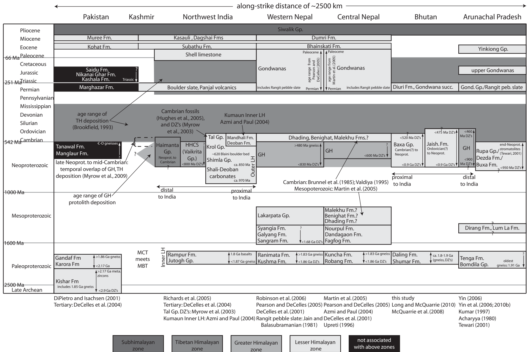
Figure 7. Correlation chart of general deposition age history of the northern Indian margin. Focus is on geochronologic and stratigraphic studies that bracket deposition ages for Lesser Himalayan units. Note along-strike continuity of Paleoproterozoic and Permian Lesser Himalayan units across all of the orogen, and presence of Neoproterozoic–Cambrian Lesser Himalayan units across much of orogen. General age brackets for deposition of Greater Himalayan protoliths, Tethyan (or Tibetan) Himalayan section (TH), and Siwalik Group shown. Note overlaps in time between Tethyan (or Tibetan) Himalayan and Greater Himalayan deposition distal to India and Lesser Himalayan deposition proximal to India. Refer to DiPietro and Pogue (2004) for a more detailed correlation chart of Lesser Himalayan units in the westernmost Himalaya. DZ—detrital zircon; GH—Greater Himalaya; HHCS— Higher Himalayan Crystalline Sequence; MBT—Main Boundary thrust; MCT—Main Central thrust; succ.—succession.
