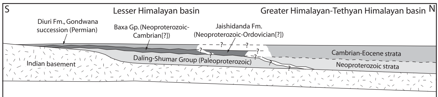
Figure 8. Schematic model for stratigraphic architecture of northern Indian margin based on Bhutan Lesser Himalayan stratigraphy. Note queried relationships of original Greater Himalayan over Lesser Himalayan contact, northern and southern extents of Jaishidanda Formation, and presence of younger Lesser Himalayan strata above Jaishidanda Formation. Note unconformity between Baxa Group and Jaishidanda Formation and underlying Daling-Shumar Group; note unconformity between Baxa Group and overlying Permian Lesser Himalayan units. Note overlap in time between Neoproterozoic–Paleozoic Lesser Himalayan deposition proximal to India and Greater Himalayan and Tethyan Himalayan deposition distal to India (note: change from light to dark gray shown for Greater Himalayan–Tethyan Himalayan basin represents change in time, and is not meant to represent the position of the stratigraphic boundary between Greater Himalayan and Tethyan Himalayan rocks).
