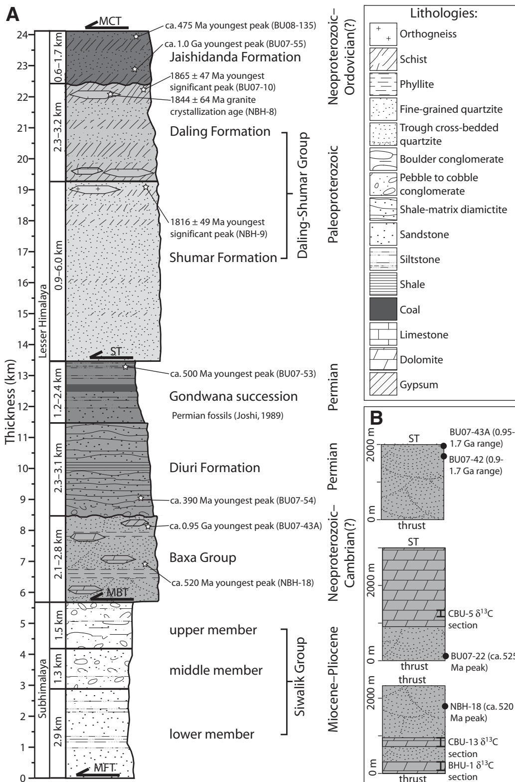
Figure 3. (A) Column showing tectonostratigraphy of Subhimalayan and Lesser Himalayan units in eastern Bhutan. Generalized lithology shown. Ages of detrital zircon peaks that constrain unit deposition are shown. Refer to Figure 1 for structure abbreviations (ST—Shumar thrust). (B) Simplified stratigraphic columns of Baxa Group sections, showing stratigraphic relationships between thrust faults, dolomite \delta^{13}C sections, and detrital zircon samples. Refer to Figure 2 for locations of detrital zircon samples and sampled dolomite intervals. Note that dolomite section CBU-5 is sampled upsection of detrital zircon sample BU07-22, which yielded a Cambrian detrital zircon peak (ca. 525 Ma). Also note that samples BU07-43A and BU07-42, which did not yield Cambrian peaks, are located near the top of the section.
