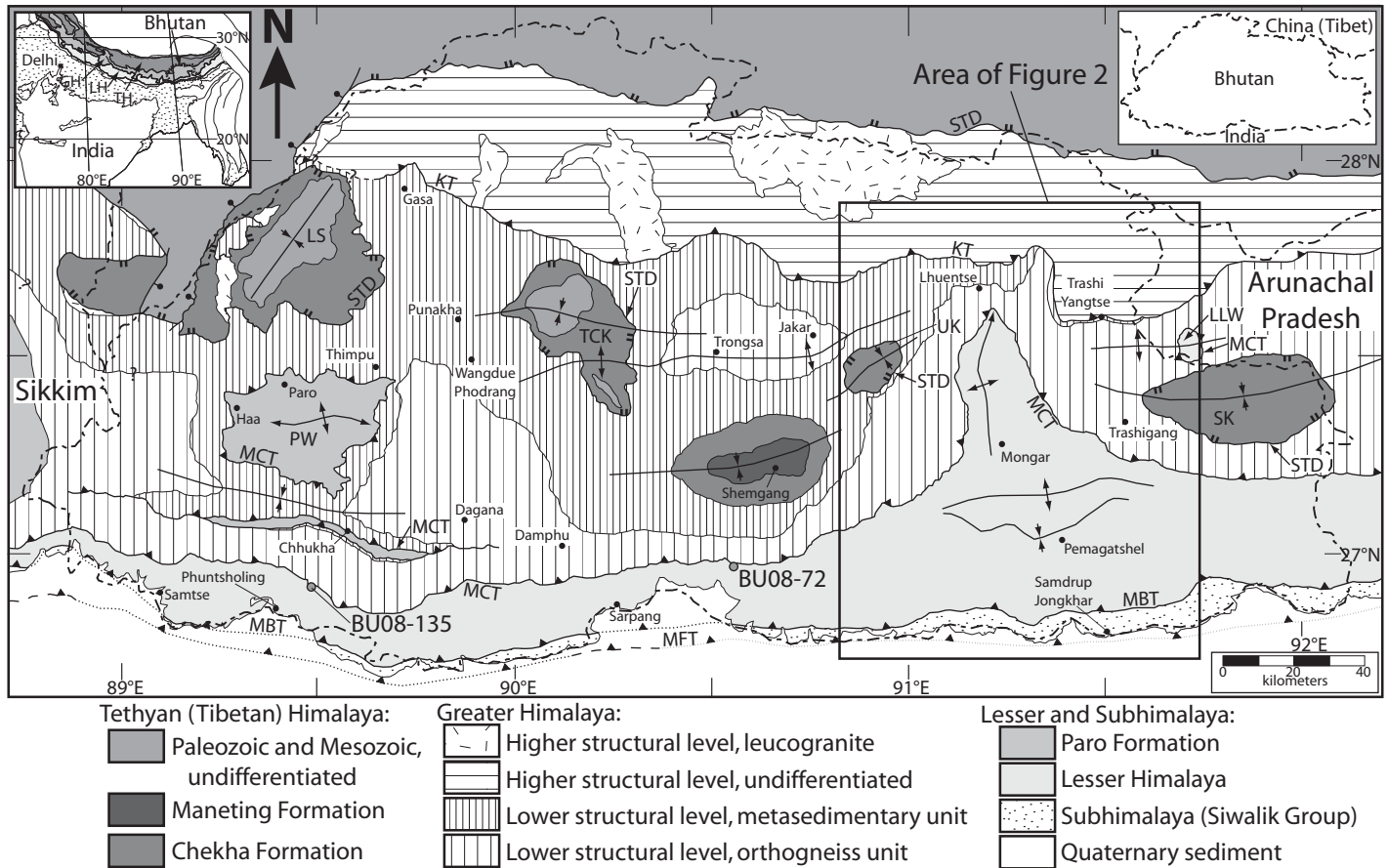
Figure 1. Simplified geologic map of Bhutan and surrounding region, after Gansser (1983), Bhargava (1995), Grujic et al. (2002), and our own mapping. Study area shown in Figure 2 outlined. Upper-left inset shows generalized geologic map of central and eastern Himalayan orogen (modified from Gansser, 1983). Structural detail left out of Tethyan Himalayan section north of Bhutan; map patterns of NE-striking, cross-cutting normal faults northwest of Lingshi Syncline (Yadong cross structure on figure 1 of Grujic et al. [2002]) are simplified. Jaishidanda Formation zircon sample locations in central and western Bhutan are shown. Abbreviations: (1) Inset: GH—Greater Himalaya, LH—Lesser Himalaya, TH—Tethyan (or Tibetan) Himalayan; (2) structures from north to south: STD—South Tibetan detachment, KT—Kakhtang thrust, MCT—Main Central thrust, MBT—Main Boundary thrust, MFT—Main Frontal thrust; (3) windows and klippen from west to east: LS—Lingshi syncline, PW—Paro window, TCK—Tang Chu klippe, UK—Ura klippe, SK—Sakteng klippe, LLW—Lum La window (location from Yin et al., 2010b).
