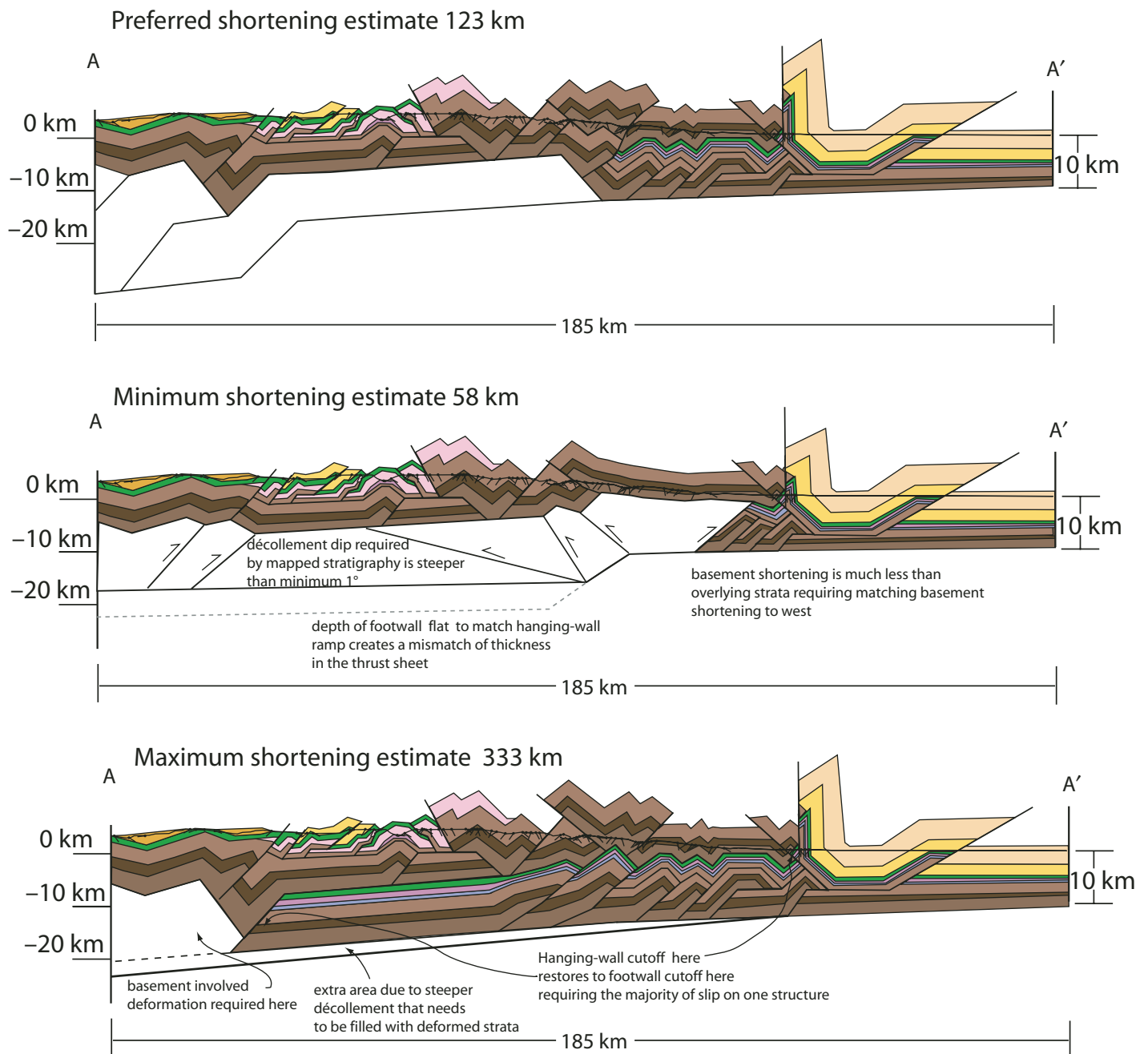
Figure 6. Variations in the way shortening is accommodated in our preferred, minimum, and maximum shortening estimates. Annotations indicate problems with the kinematics in the maximum and minimum shortening estimates. Stratigraphic color key is given in Figure 2.
