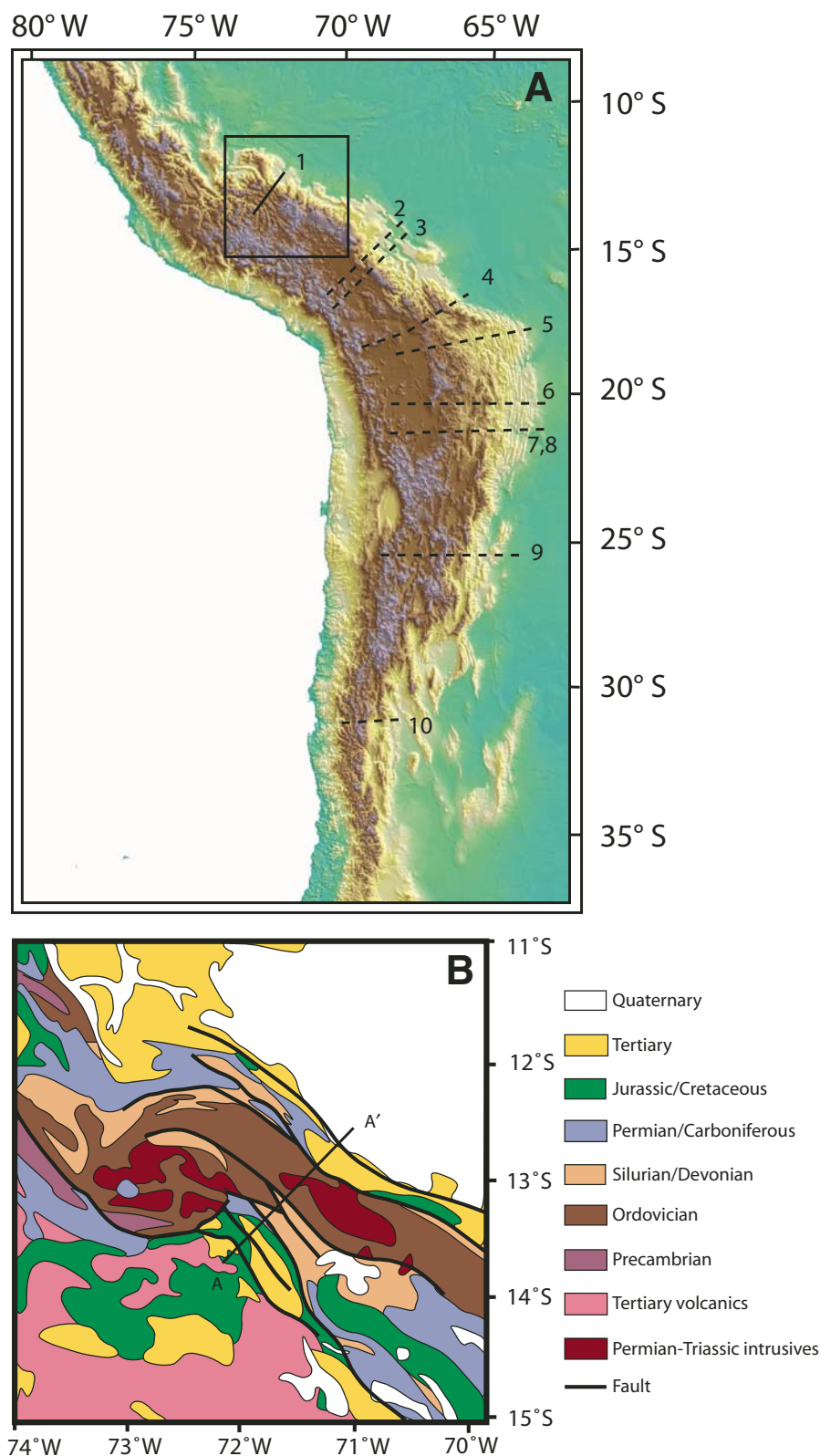
Figure 1. (A) Color topography of the Andean Plateau and the Bolivian orocline. Box indicates location of B and the study area. Black line represents the location of the cross-section line. Numbers and dashed lines refer to cross sections discussed in text and in Figure 8. The northern boundary of the Altiplano is located within the black box. (B) Generalized geologic map of the northern margin of the Andean Plateau.
