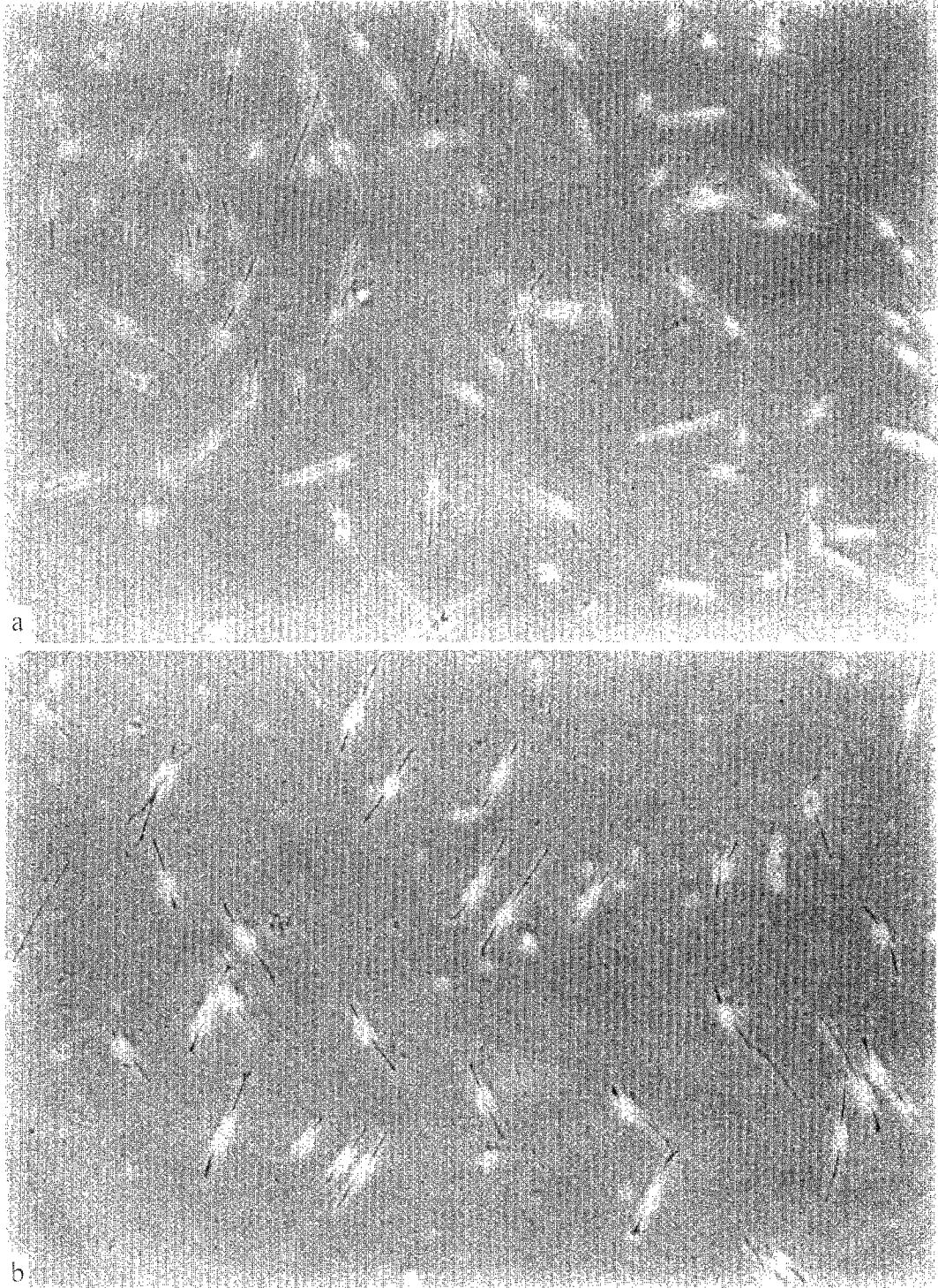
Fig. 3. (a) Photomicrograph ( 50\times ) of human melanocytes grown at low density in the absence of a stretch stimulus. (b) A similar population of cells grown on a substrate subjected to a 1 Hz 12% peak-to-peak applied stretch for 24 h. Note that the cells tend to align at 60^\circ to the applied stretch direction (horizontal), near the direction of zero axial surface strain.
