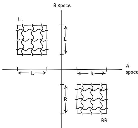
Fig. 6. Configuration space of two correlated particles of boxes A and B.
