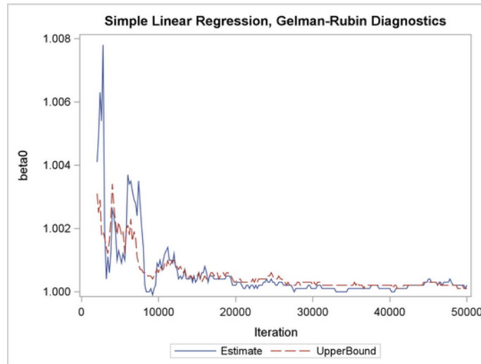
Figure 3: A Markov Chain Monte Carlo Converging on a Stable Estimate
