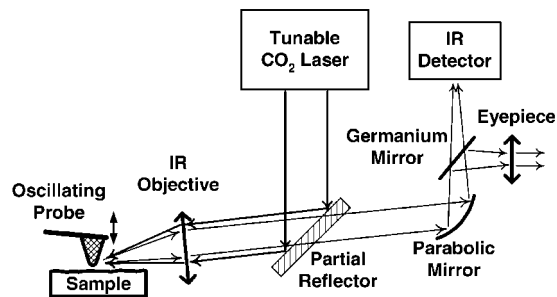
Figure 1. A schematic of the apertureless near-field infrared microscope.
