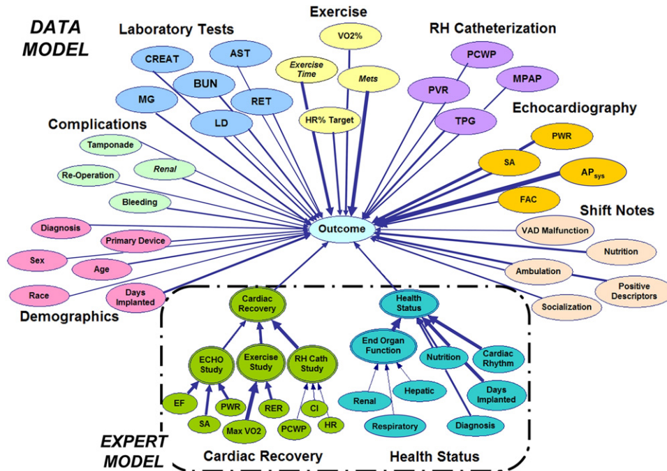
Fig 3. Hybrid Bayesian belief network model combining expert and data models. (See the Abbreviations List for expansions of the abbreviations.)
