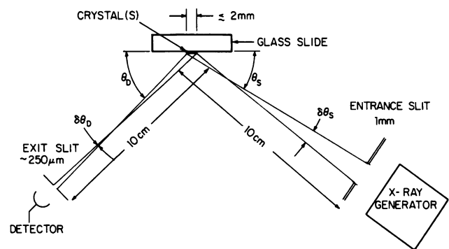
FIG. 4. Schematic of the x-ray diffractometer. For (\theta, 2\theta) scans, \theta = \theta_s = \theta_D . For \omega scans, \theta_s + \theta_D is held fixed and \omega = (\theta_s - \theta_D)/2 .
