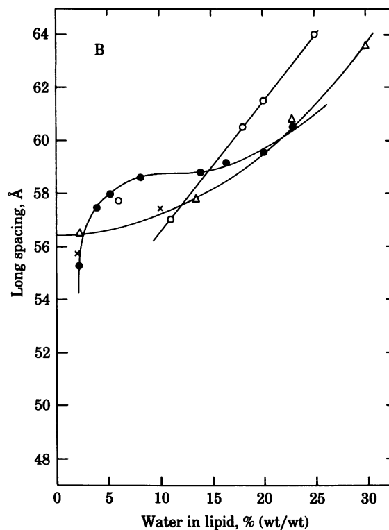
FIG. 3. X-ray measurements of the hydration of a Pam 2 PtdCho crystal at 20°C. (A) Long spacing as a function of relative humidity. Points ( \Delta ) were recorded in the sequence indicated. \times indicates data by Torbet and Wilkins (22). (B) Same data as in A expressed in terms of weight percent of absorbed water by using Elworthy's (32, 33) measured relationship to RH. \bullet , our data; \circ , Tardieu et al. (14); \Delta , Chapman et al. (13); \times , Stamatoff et al. (19). We assume that overnight exposure to pure H 2 SO 4 produces the monohydrate.
