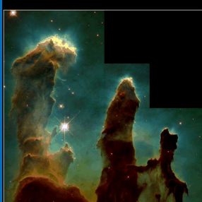
Gaseous Pillars - M16 HST - WFPC2 PRC9044a - ST ScI 090 - November 2, 1995 J. Hester and P. Scovren (AZ State Univ.), NASA
